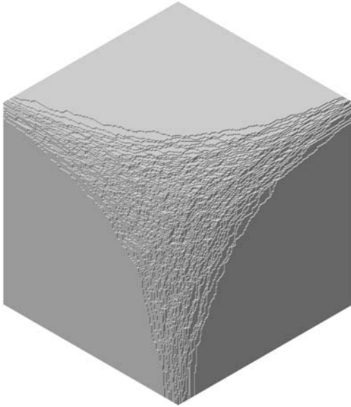
Fig. 1. Crystal corner viewed from the (111)-direction for q = 0.98 .
