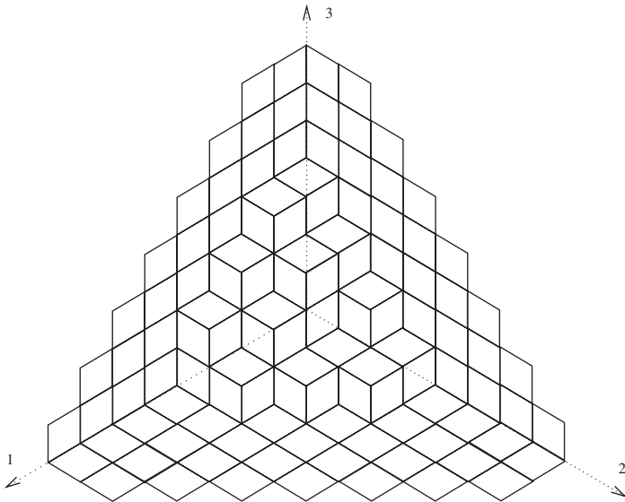
Fig. 2. The (111) projection of a configuration n \in \Omega . In each of the three sectors the tiling becomes regular far away from the origin.
