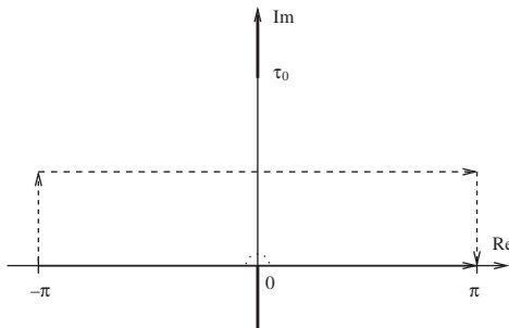
Fig. 7. Deformation of the integration path. The original integral, from -\pi to \pi , is deformed along the integral on the dashed path.
