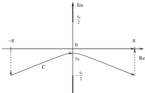
Fig. 9. Deformation of the integration path. The path from -\pi to \pi is deformed into C plus the dashed ones.
